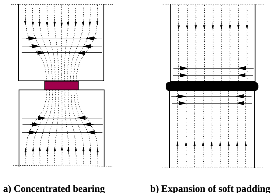
Figure 10.3: Transverse tensile stresses at compression connections.
