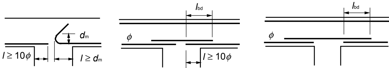
Figure 9.4: Anchorage at intermediate supports
